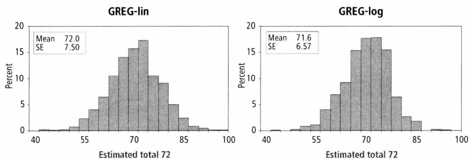
Figure 6.3 Histogram of GREG-lin and GREG-log under the SRSWOR design.
