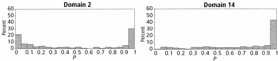
Figure 5.3 Histograms of p = P(\underline{y}_3 = 1) in selected domains of Population 1.
