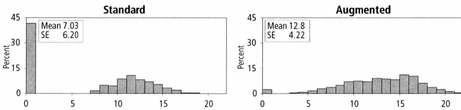
Figure 7.6 Histograms of Standard and Augmented variance estimators. \pi PS design, size variable z_1 , n=40 , population level estimates, GREG-log, set 9. True standard error 17.3.
