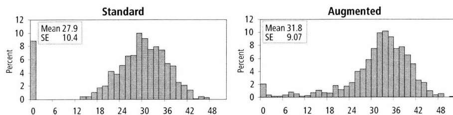
Figure 7.3 Histograms of Standard and Augmented variance estimators. SRSWOR design, n=1,000 , domain 15 (medium), estimator set 4, GREG-log. True standard error 33.4.
