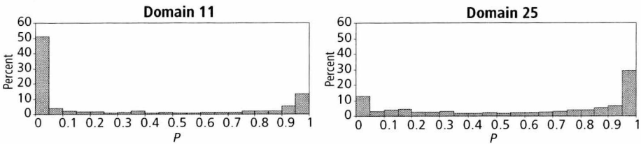
Figure 5.2 Histograms of p = P(\underline{y}_2 = 1) in selected domains of Population 1.
