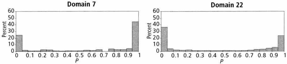
Figure 5.1 Histograms of p = P(\underline{y}_1 = 1) in selected domains of Population 1.
